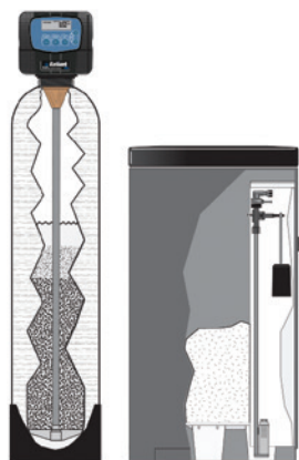
Resin Scrubber Vortech™ Design: VT Model
